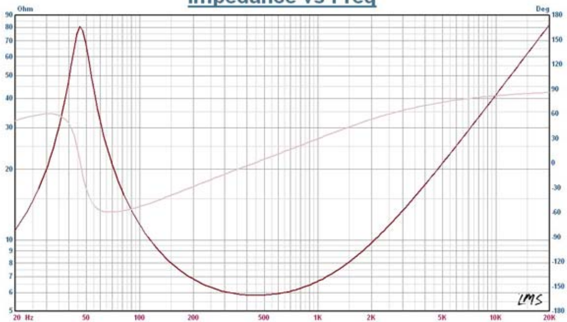
Impedance vs Freq
